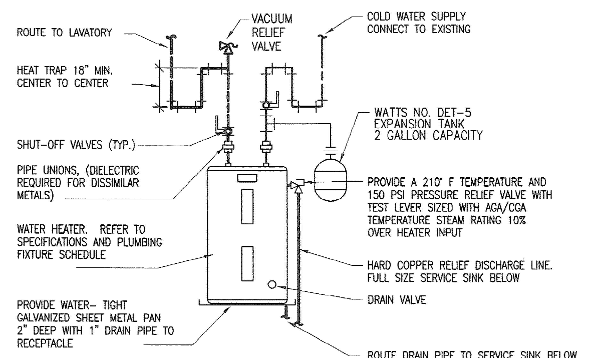
2 WATER HEATER DETAIL SCALE: NOT TO SCALE
