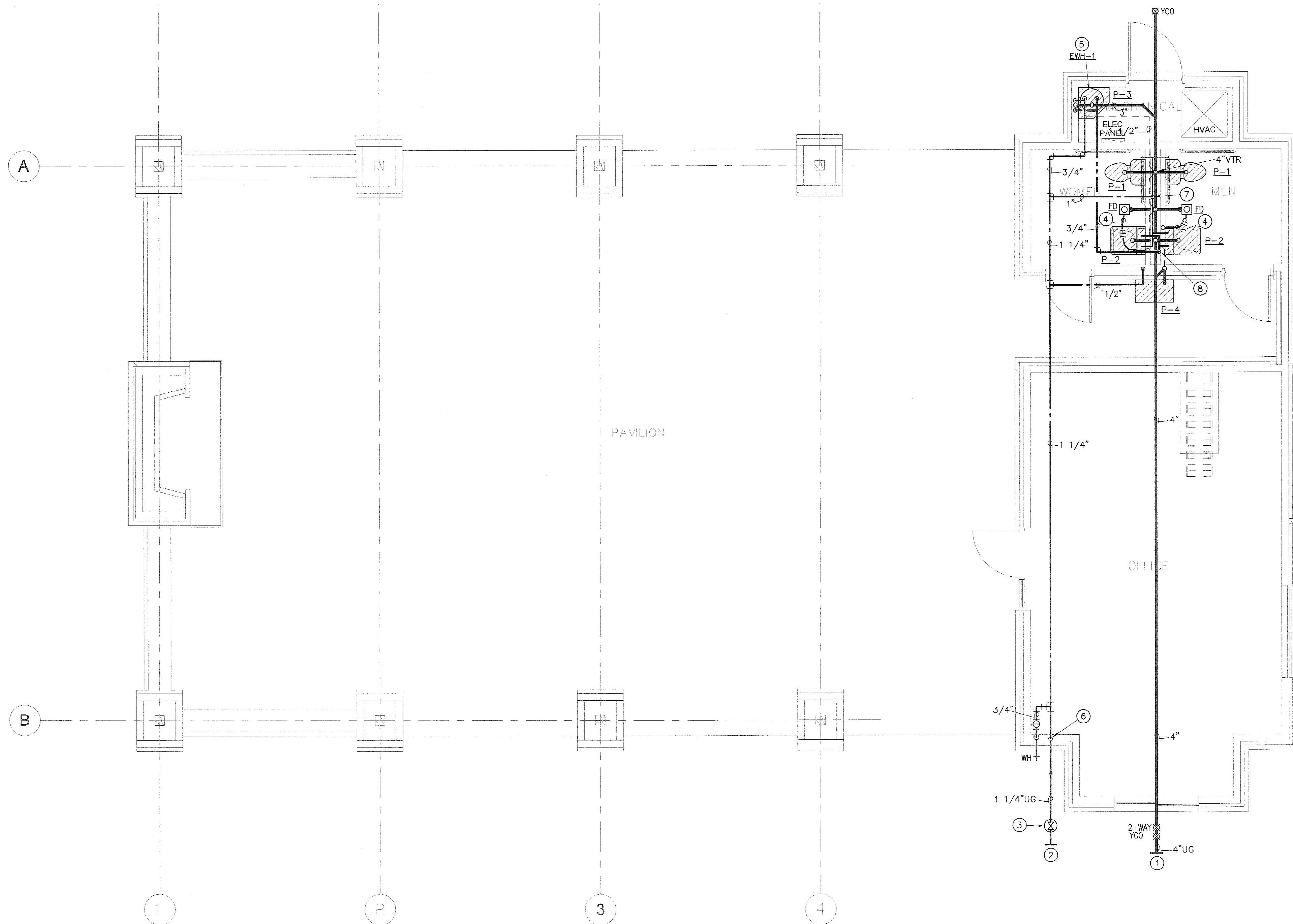
1 PLUMBING FLOOR PLAN SCALE: 1/4"=1'-0"
