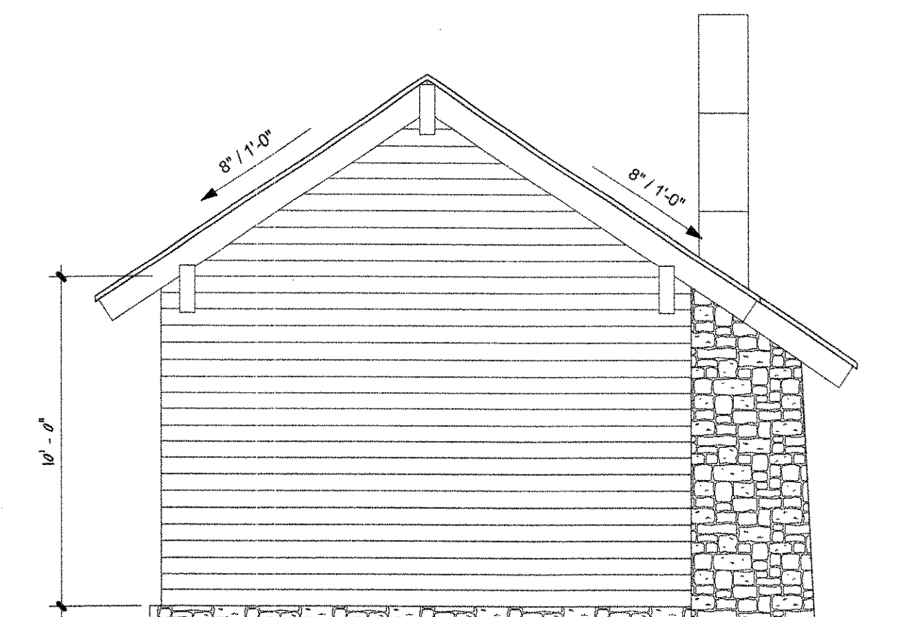
4 SOUTH ELEVATION - POOL HOUSE SCALE: 1/4" = 1'-0"
