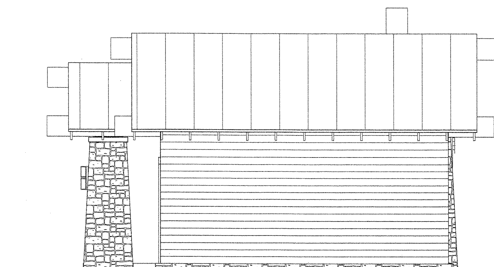
5 EAST ELEVATION - POOL HOUSE SCALE: 1/4" = 1'-0"
