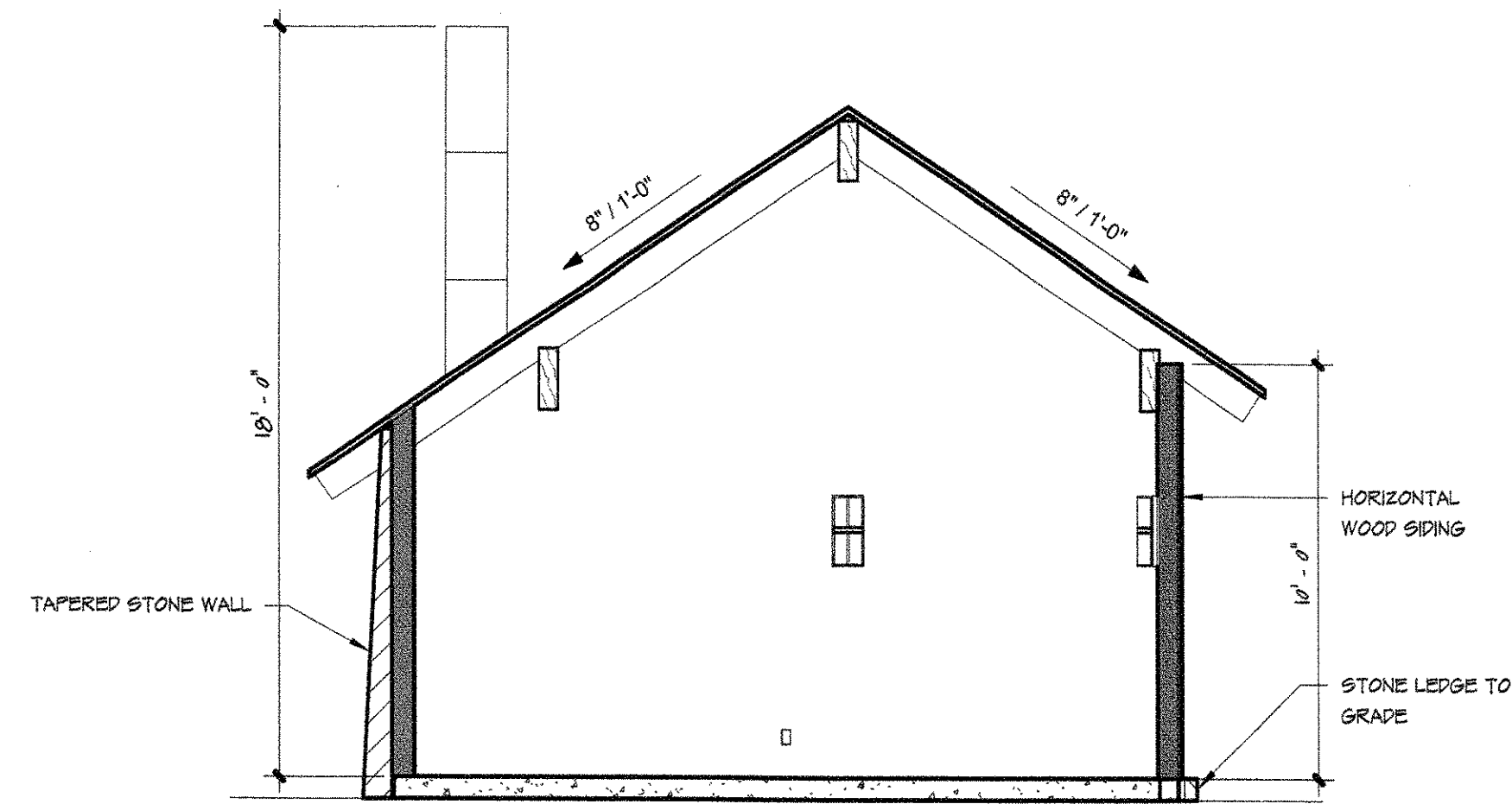
7 BUILDING SECTION SCALE: 1/4" = 1'-0"
