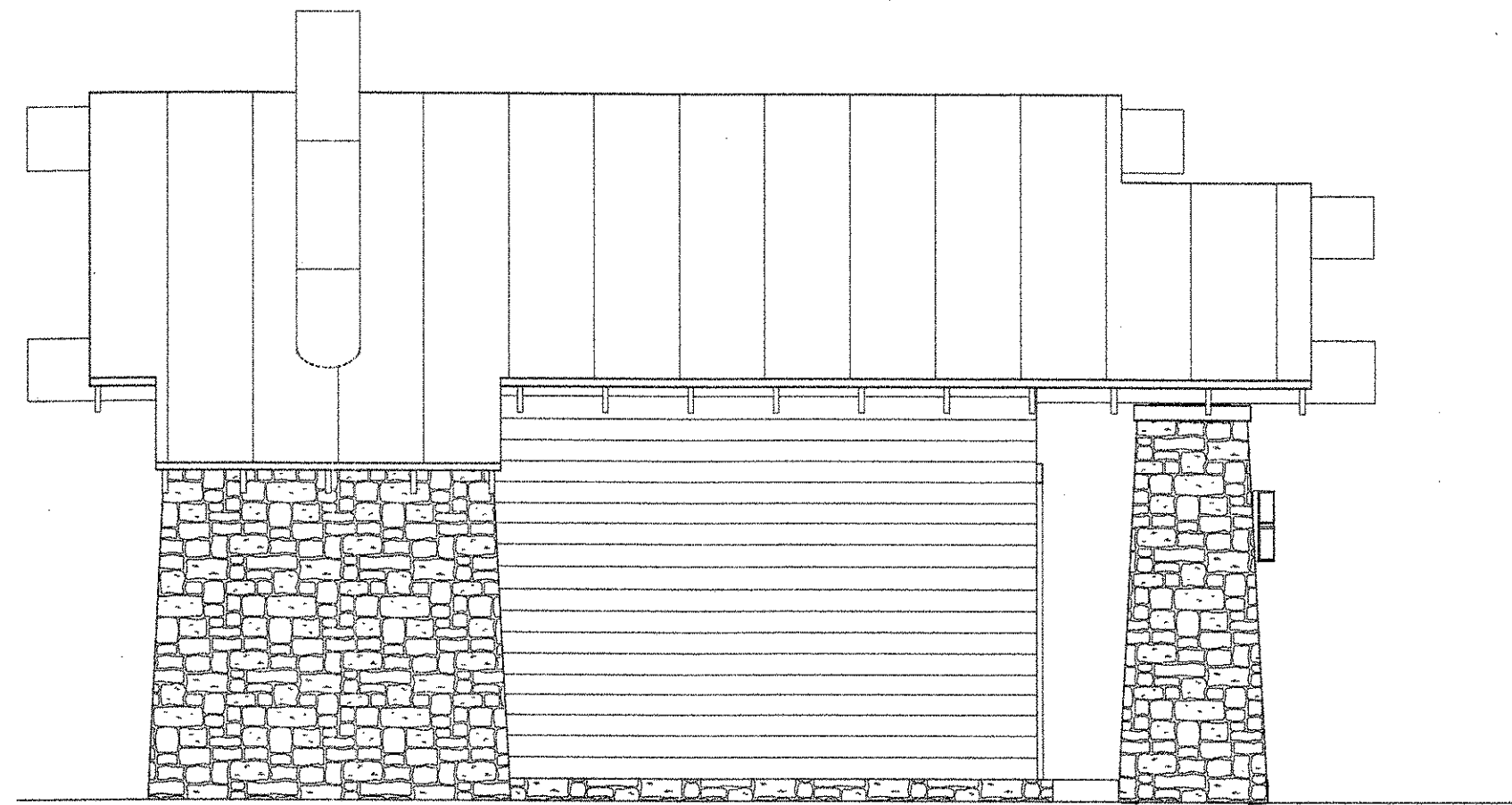
4 SOUTH ELEVATION - POOL HOUSE SCALE: 1/4" = 1'-0"
