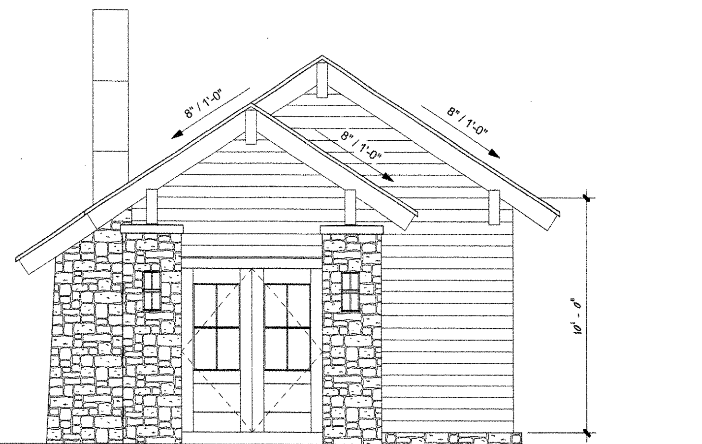
5 EAST ELEVATION - POOL HOUSE SCALE: 1/4" = 1'-0"
